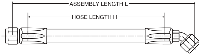
Straight-To-45° Elbow
