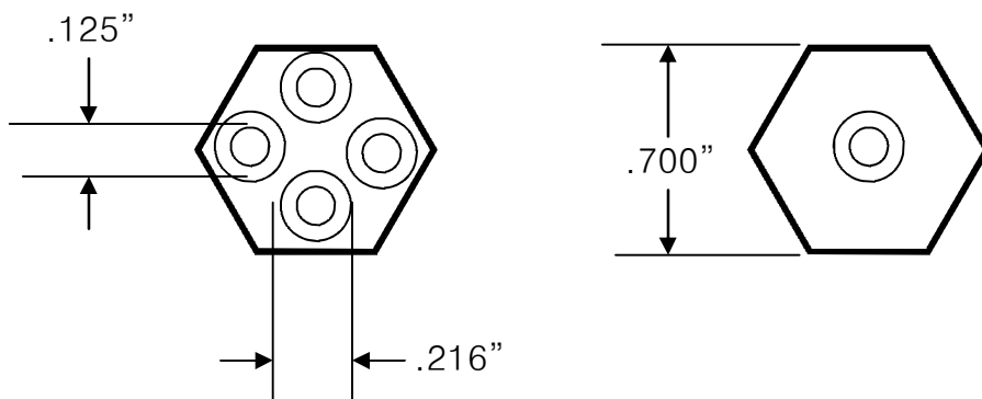
SIDE VIEW OF CAP NUTS
